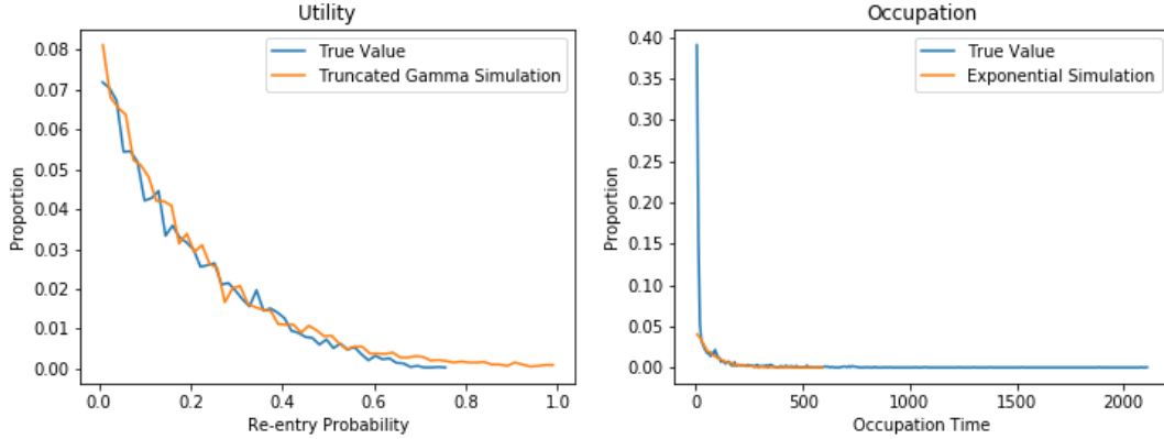
Figure 4: Performance of simulators for re-entry probability (matching utility) and occupation time
