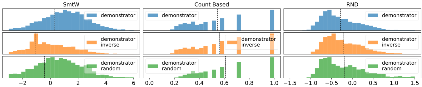
Figure 6: Bonus distribution received by the demonstrator behavior (top), the inverse demonstrator behavior (middle), and the random demonstrator behavior (bottom).
