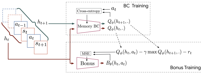
Figure 1: Trajectories (s, a, \dots) are generated by a demonstrator exploring its environment. In order to recover a bonus that can explain its behavior, a BC policy parameterized with an LSTM is trained to predict the actions of the demonstrator from its trajectories of states, by minimizing \mathcal{L}^{\text{BC}} . The policy’s logits Q_\phi are interpreted as optimal Q -values and used to compute a regression target. A bonus function B_\theta , parameterized with an LSTM, is then trained to predict it, by minimizing \mathcal{L}^{\text{reg}} .
