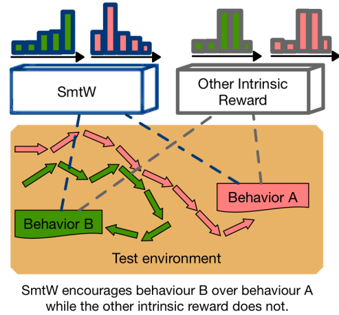
Figure 2: Comparing intrinsic rewards on what behavior they encourage or discourage on new unseen environments.
