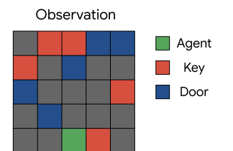
Figure 3: KeysDoors(N=5).
