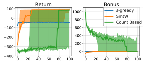
Figure 11: Median and min/max values of the return per episode (left) and of the total bonus per episode(right).
