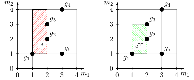
Figure 1: Non-closed (left) and closed (right) interval pattern.
