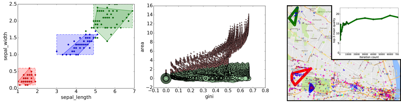
Figure 8: Comparing interval and convex polygon top-3 patterns (Left). Comparing interval and convex polygon patterns gini, area and density (Center). Top-3 homogeneous convex polygon patterns on Foursquare places from Saint-Louis (Missouri, USA) (Right).
