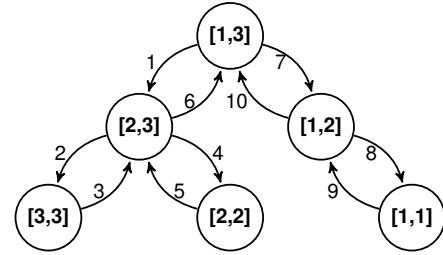
Figure 2: Depth-first traversal of (D_{m_1}, \sqcap) .
