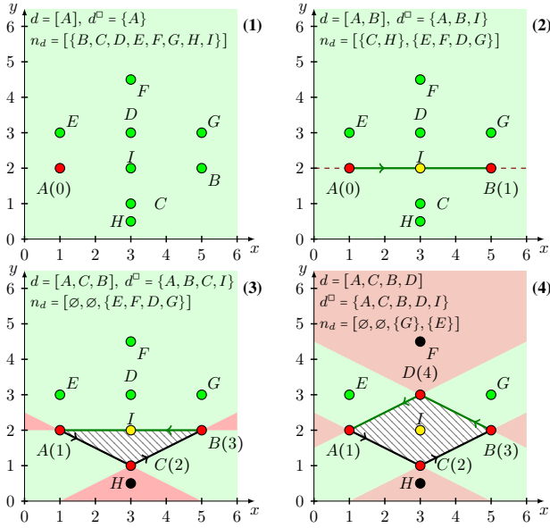
Figure 5: EXTREMEPOINTS ENUM algorithm step-by-step enumeration.
