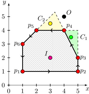
Figure 3: Convex polygon and edges visibilities.
