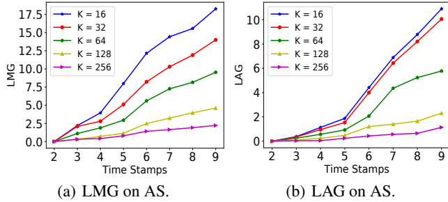
Figure 2: Metric values on AS with different K values. The left sub-figure shows the values of LMG, while the right one shows those of LAG. Each curve represents a K value. Usually, the larger the K , the lower the LMG and LAG.
