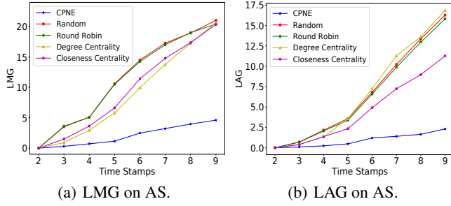
Figure 1: Metric values on AS. The left sub-figure shows the values of LMG, while the right one shows those of LAG. Each curve represents an algorithm. For both two metrics, the smaller the metric value, the better the algorithm.
