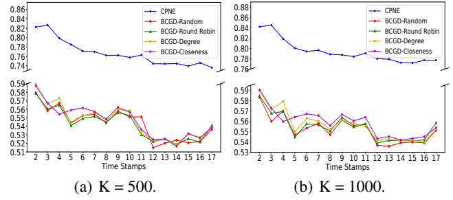
Figure 3: AUC values at each time stamp on WeChat dataset.
