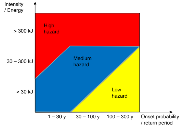
Fig. 4. Hazard classification for rockfall in Switzerland
