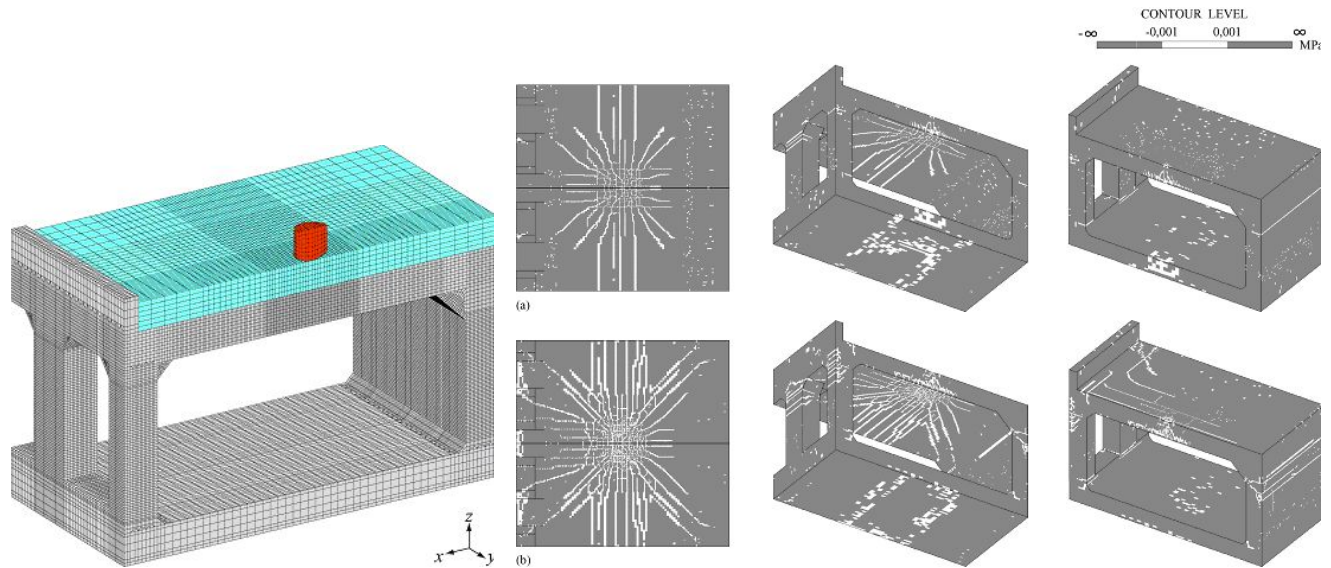
Fig. 17. General view of an FE analysis model of an impacted rock shed and the resulting crack patterns for different loading cases (from Kishi et al., 2009).
