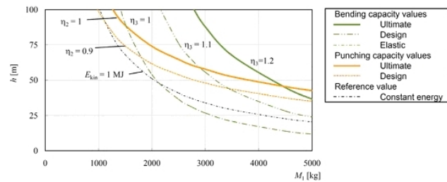
Fig. 16. Loading capacity of protection gallery Axen-Süd for different impact masses (from Schellenberg, 2009).
