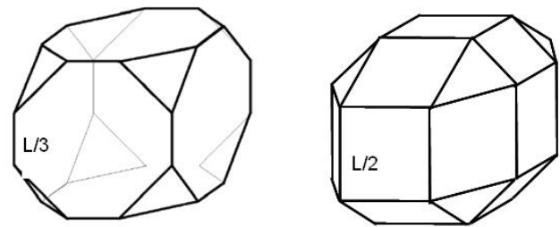
Fig. 21. Standardized test blocks for flexible rockfall protection systems related to a regular cube with edge length L according to the approval guidelines of Switzerland (left, Gerber, 2001a, until 2008) and the European Union (right, EOTA, 2008).
