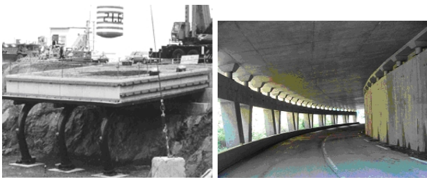
Fig. 12. Full-scale steel-concrete composite rock shed subjected to a falling weight (left; Maegawa et al., 2003), gallery with PSD dissipation system in Val d’Arly, France (right; taken from Masuya, 2007).
