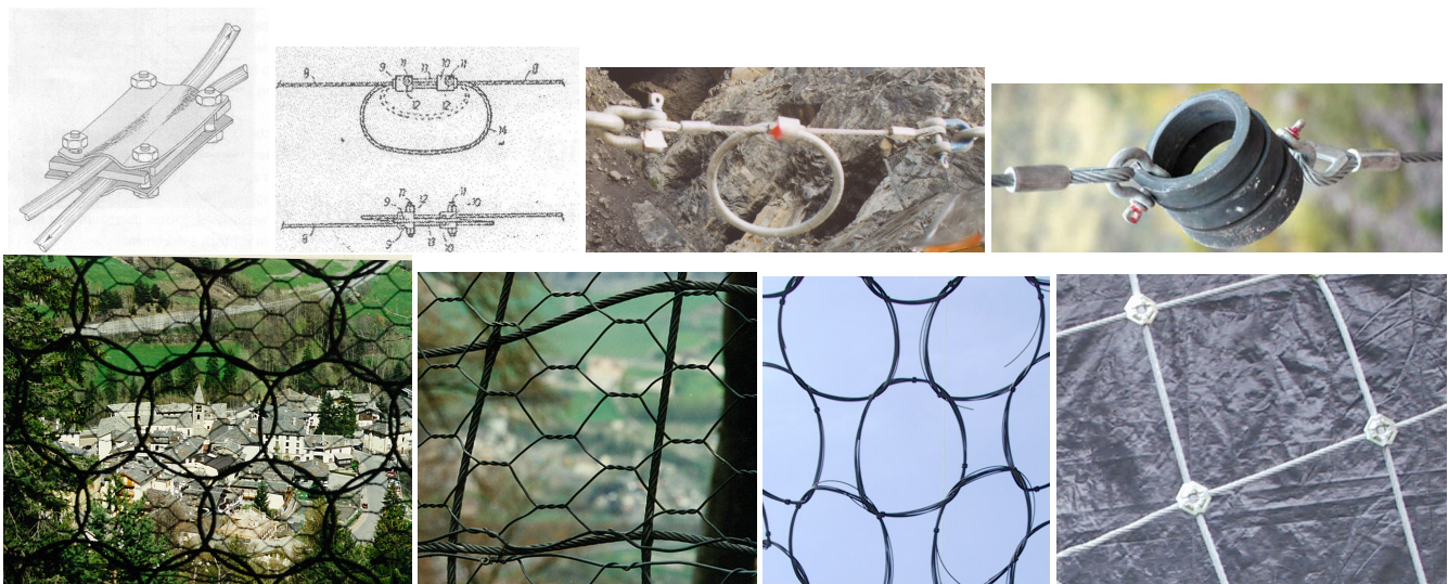
Fig. 18. Different types of energy absorbing barrier components (friction of tensioned rope between friction plates, friction between rope clamps, bent steel pipe circle narrowing under tension and elongating spiral structures) and mesh types (original anti-submarine net, hexagon mesh and spliced rope net, ring net, rope net with clamps).
