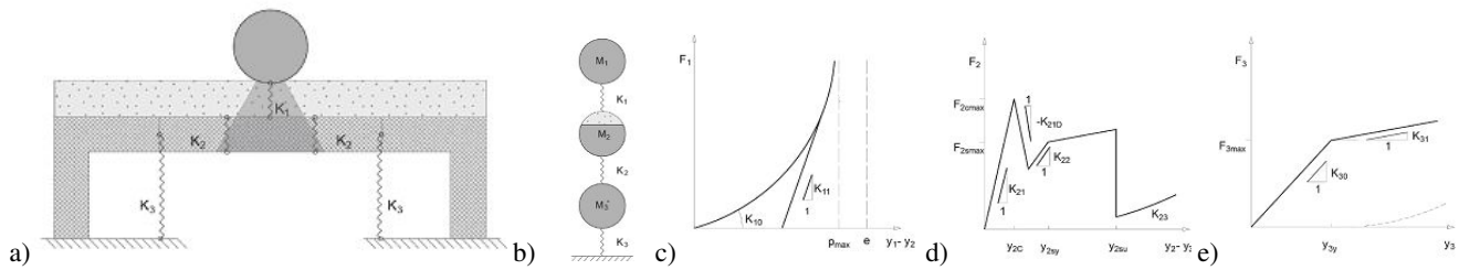
Fig. 15. System with multiple degrees of freedom (SMDF) (a) and (b), from the section of a gallery to the model definition together with the force-displacement relationship of the springs for (c) cushion layer, (d) shear behaviour and (e) global bending stiffness (from Schellenberg and Vogel, 2009).
