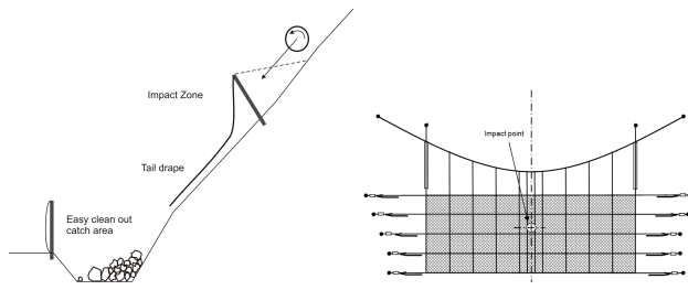
Fig. 19. Principle mode of operation for rockfall attenuating system (left, Glover et al., 2010) and system sketch for typical hanger net system (right).
