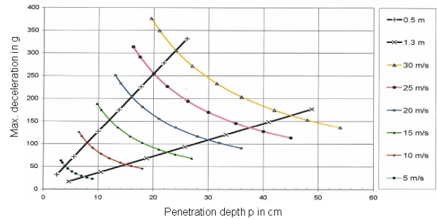
Fig. 10. Penetration and deceleration of impacting rocks onto consolidated soil of thickness 0.5 m and 1.3 m for different impact velocities.
