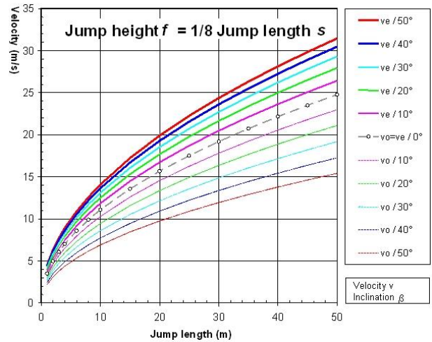
Fig. 9. Lift-off and impact velocity for an assumed jump height of f/s = 1/8 as a tool for rapid trajectory analyses in the field.
