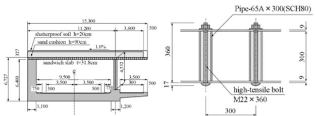
Fig. 13. Steel-concrete composite structure for a rockfall protection gallery (Konno et al., 2008)
