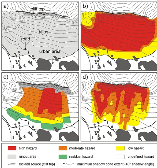
Fig. 3. Comparison of hazard maps derived for the area of Mt. S. Martino (Lecco, Italy; Jaboyedoff et al., 2001; Crosta and Agliardi, 2003) using different modelling approaches and zoning methods. (a) Maximum runout area estimated by a shadow angle approach using the code CONEFALL (Jaboyedoff and Labiouse, 2003); (b) hazard map obtained by applying the RHV methodology (Crosta and Agliardi, 2003) to the reach probability and kinetic energy estimated by CONEFALL; (c) rockfall hazard map obtained by 2-D numerical modelling using the RHAP methodology (modified after Mazzoccola and Sciesa, 2000); (d) rockfall hazard map obtained by 3-D numerical modelling using the code HY-STONE and the RHV methodology (modified after Crosta and Agliardi, 2003).
