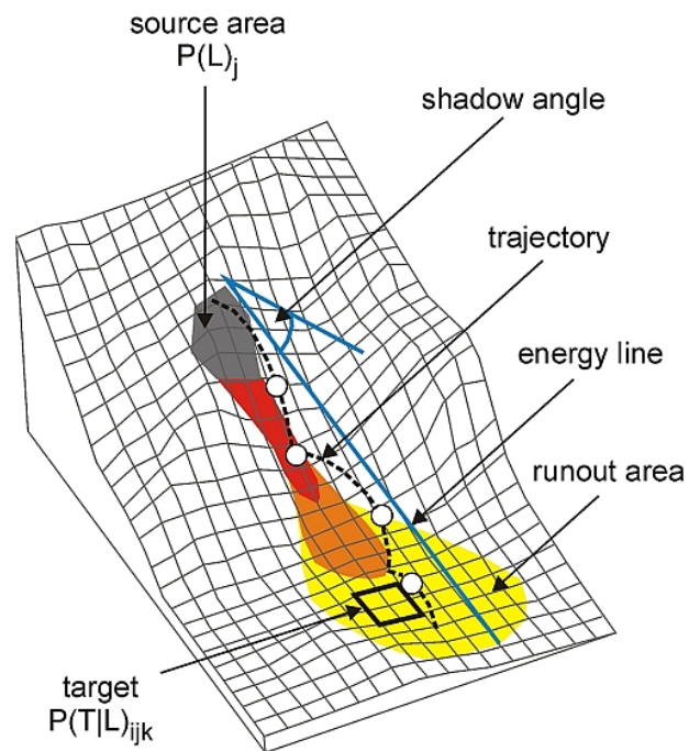
Fig. 2. Definition of rockfall hazard and related parameters (modified, after Jaboyedoff et al., 2001).
