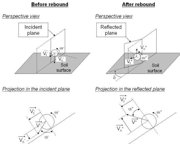
Fig. 6. Definition of the block velocity before and after rebound.
