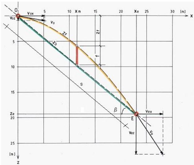
Fig. 8. Details of air parabola with velocity vectors.
