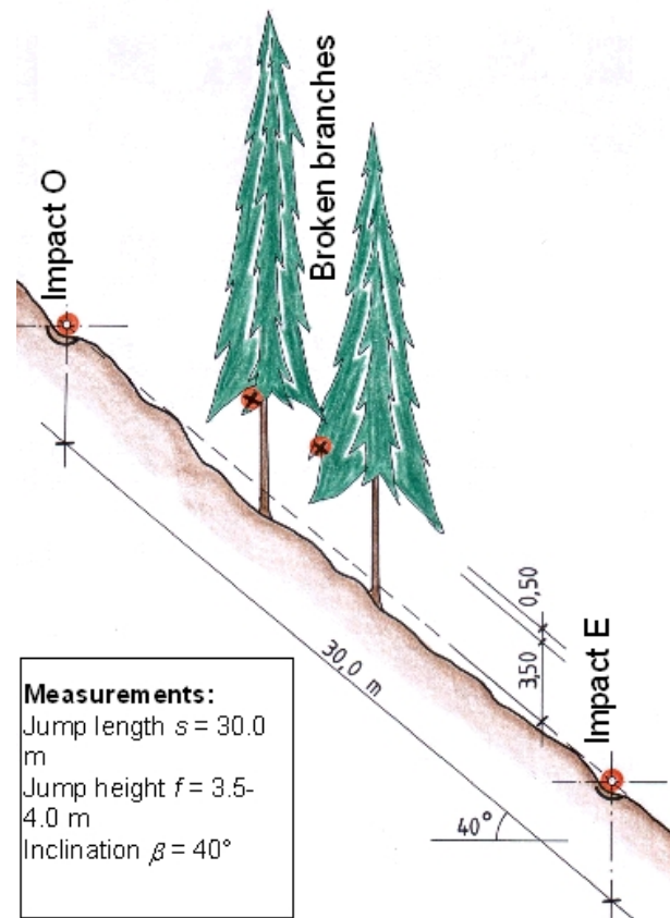
Fig. 7. Schematic illustration of rockfall traces on the ground and tree branches.
