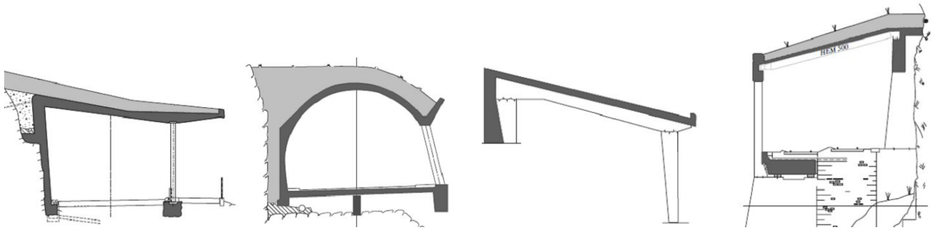
Fig. 11. Different types of shed structures (fltr): reinforced-concrete slab, shell type, in situ reinforced concrete, and steel-concrete-composite type (from Vogel et al., 2009).
