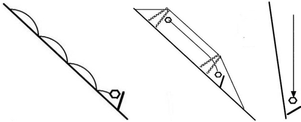
Fig. 20. Different testing methods for rockfall protection systems: free trajectory (left) with impact including rotation, but imprecise impact location; cable car guided oblique (middle) and vertical (right) impact with precise impact location.
