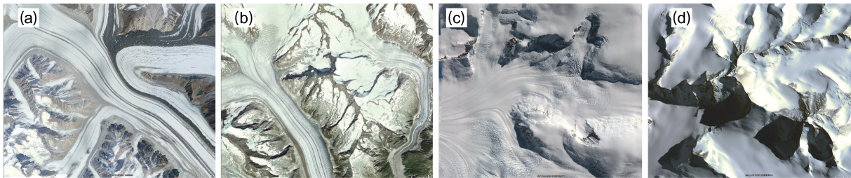
Figure 4. Comparison of debris cover for glaciers at low latitudes: (a) Karakoram Range (35° N) and (b) Jungfrau Range, Alps (46° N), with those of Antarctica (c), the Antarctic Peninsula (66° S) and (d) Transantarctic Mountains (72° S). Note the lack of surface moraine and the deep shadows in (c) and (d), typical of Antarctic glaciers where a lack of day–night cycle and year-round low temperatures restricts freeze–thaw action and the permanently low sun angles result in deep shadows in remotely sensed imagery.
