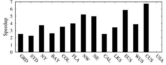
Figure 8: TL-Query speedup over HL-Query.
