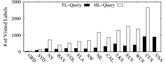
Figure 9: Number of visited labels in query processing.
