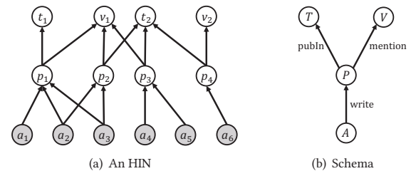
Figure 1: An example HIN with a star-schema.
