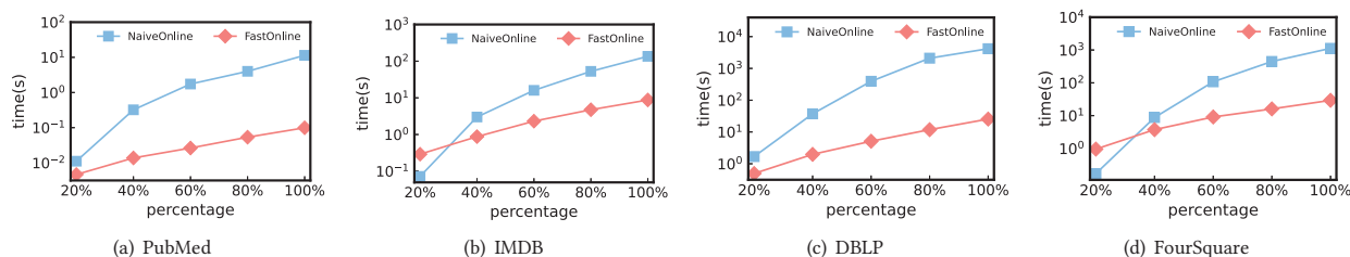
Figure 8: Scalability test for online query algorithms.
