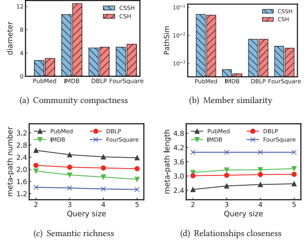
Figure 6: Results of effectiveness evaluation.
