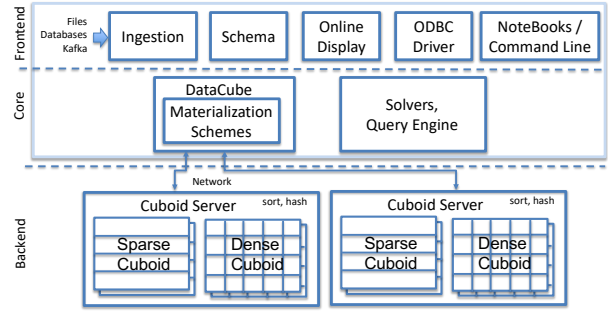
Figure 6: Sudokube architecture
