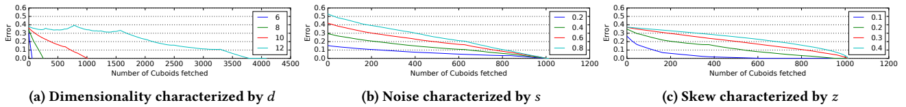
Figure 11: Impact of various data distribution parameters of the microbenchmark on the moment solver error in online mode.
