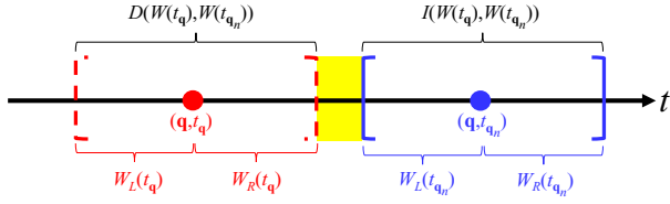
Figure 24: The case for t_{q_n} - t_q > \frac{2}{\gamma_t} .
