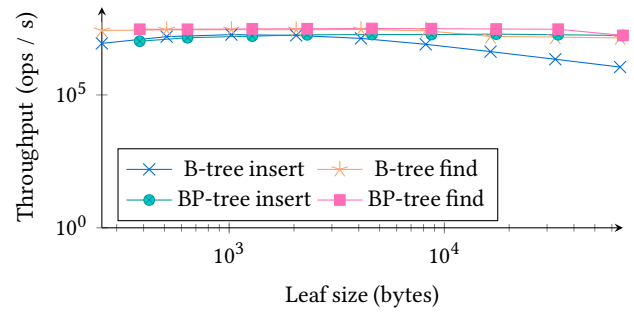
Figure 5: Point operation throughput as a function of leaf size.
