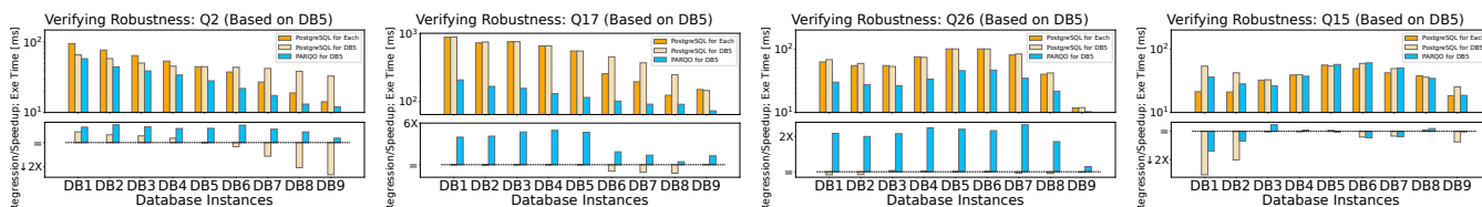
Figure 3: Actual execution times of JOB queries on multiple instances by time-slicing IMDB. DB5 is the base instance.
