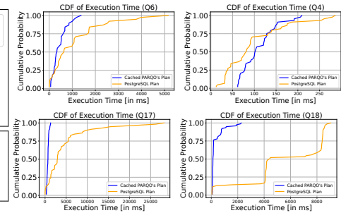
Figure 7: Cumulative density function of execution time in PQO: for Q6, Q4, Q17 and Q18
