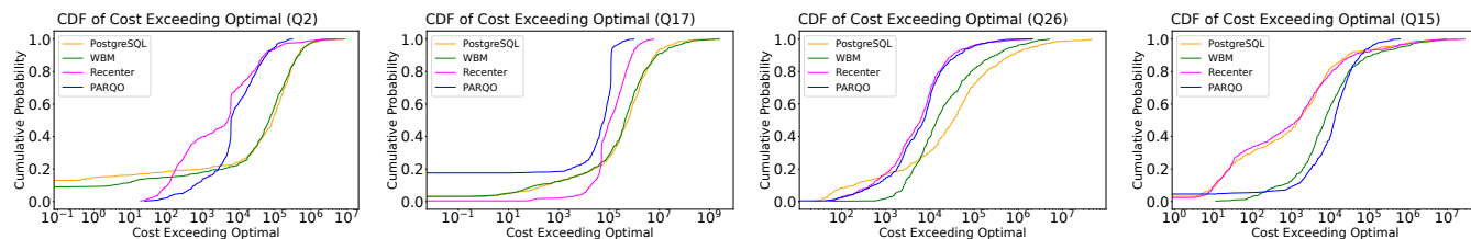
Figure 2: Cumulative density of cost exceeding the optimal by plans for Q2, 17, 26 and 15 in JOB.
